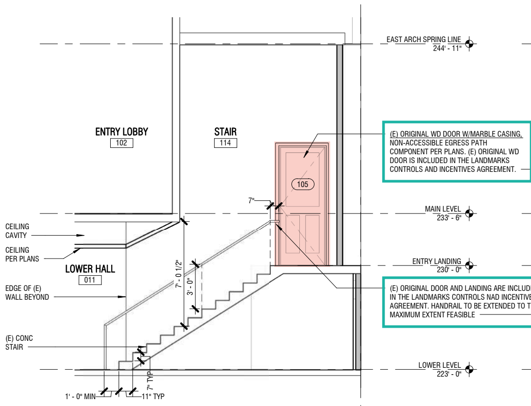
LOWER LEVEL STAIR SECTION
