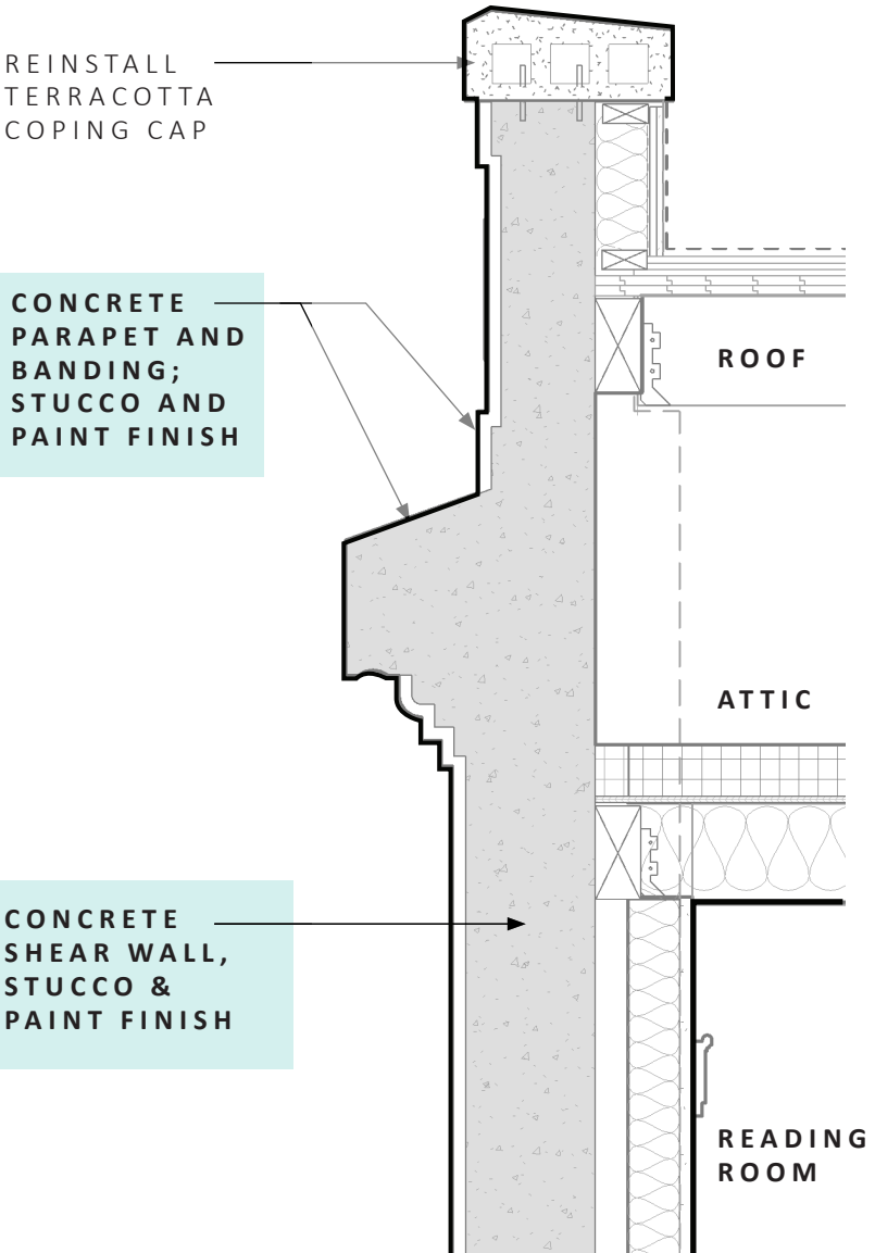
NORTH/SOUTH WALL SECTION
