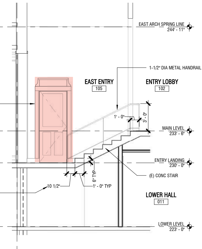
MAIN LEVEL STAIR SECTION
